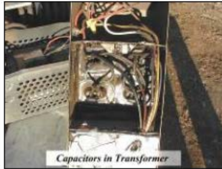
Prohibited: Capacitors in transformer
